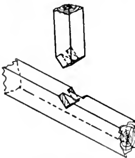
FIG. 17.—Bridle Joint.
