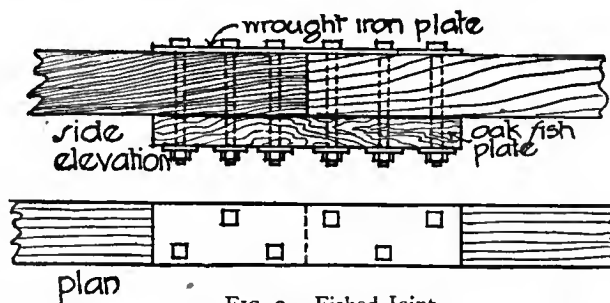
FIG. 2.—Fished Joint.
