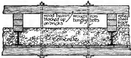
FIG. 20.—Method of supporting Centering for Concrete.
