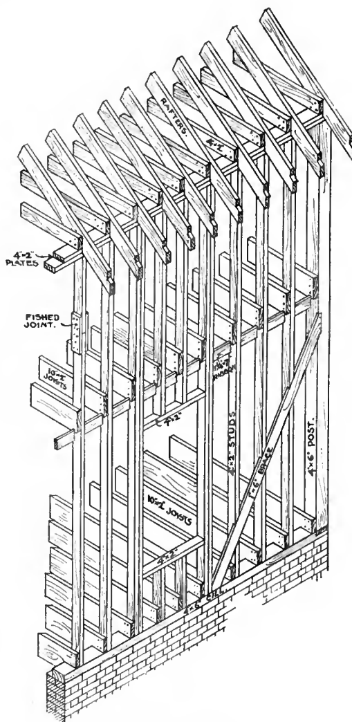
FIG. 36.—Balloon Frame.
