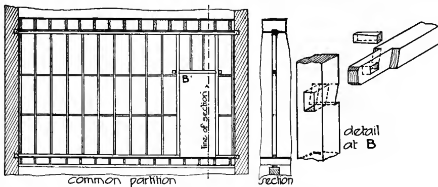
FIG. 30.—Common Partition.
