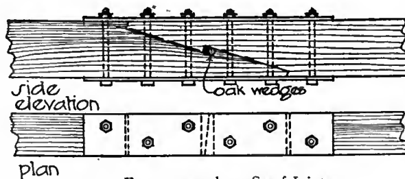
FIGS. 3, 4 and 5.—Scarf Joints.
