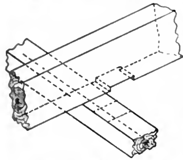
FIG. 6.—Notching.
