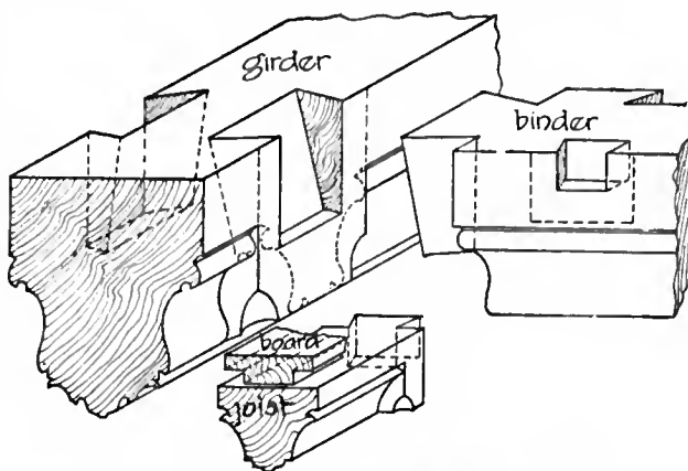
FIG. 27.—Construction of a Medieval Floor.
