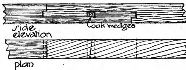
FIG. 2.—Fished Joint.
