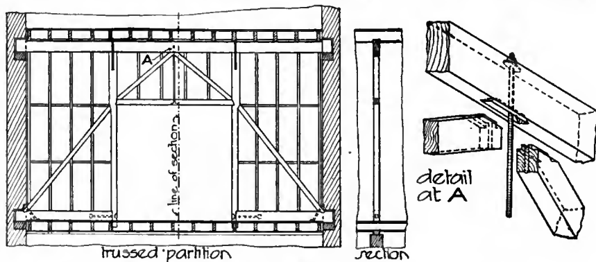
FIG. 31.—Trussed Partition.
