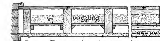
FIG. 24.—Floor pugged to resist passage of sound.
