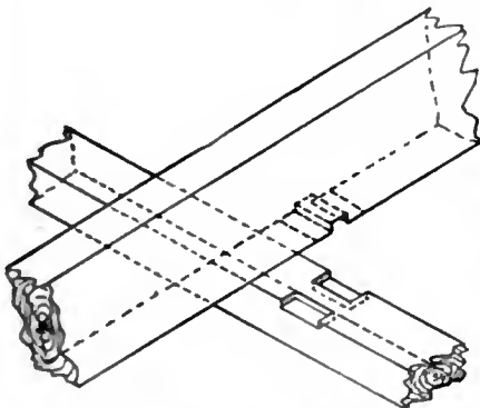
FIG. 7.—Cogging.
