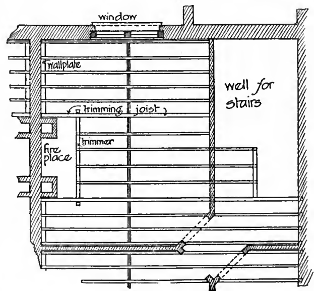
FIG. 23.—Single Floor.
