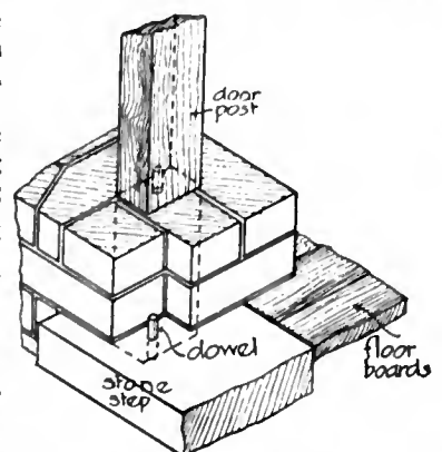
FIG. 19.—Dowelling.
