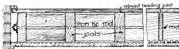
FIG. 29.—Solid Strutting.
