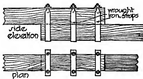
FIG. 1.—Lapped Joint.
