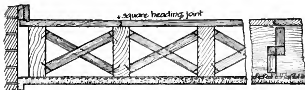
FIG. 28.—Herring-bone Strutting.
